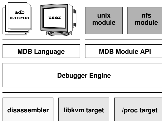
Figure 2.1: MDB architecture
